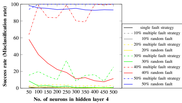
Fig. 5: Target activation function – tanh.
